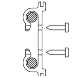
Fig. 2 - Top view of wire retention clamps
